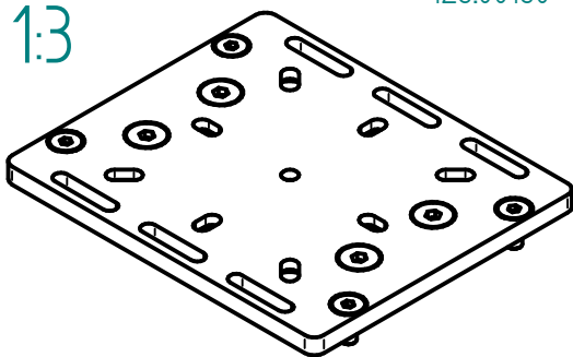
Adapterplatte SN SNT 40 45 Adapter plate SN SNT 40 45 126.00160
