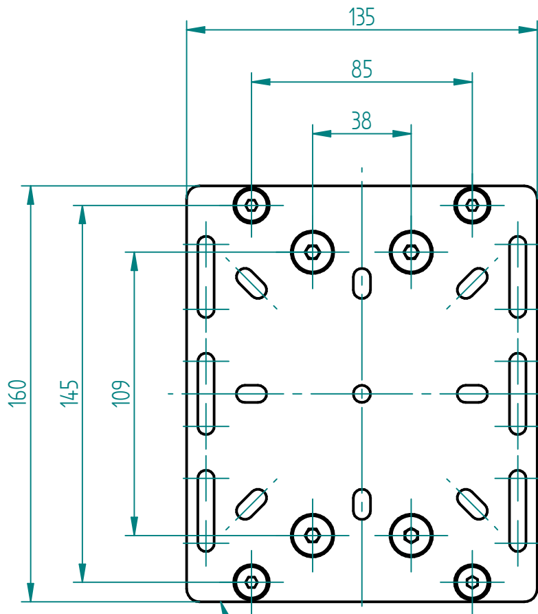
Adapterplatte SN SNT 40 45 Adapter plate SN SNT 40 45 126.00160
