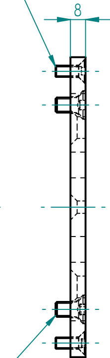
Senkschraube M6x16 Countersunk screw M6x16 142.00082 (4x)
